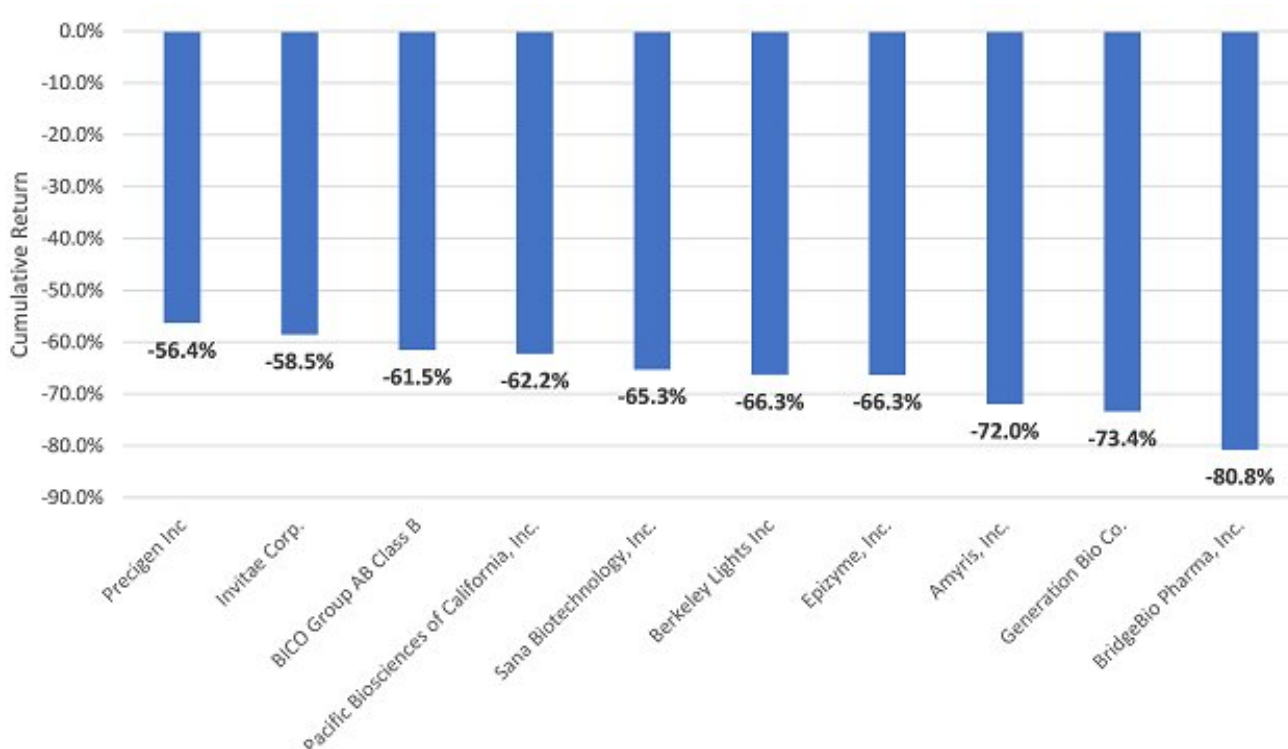
Figure 1: Cumulative Returns (7 November 2021 to 7 February 2022)
