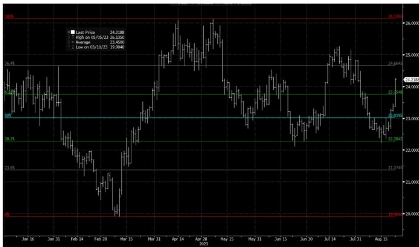
Figure 2: Fibonacci retracements
