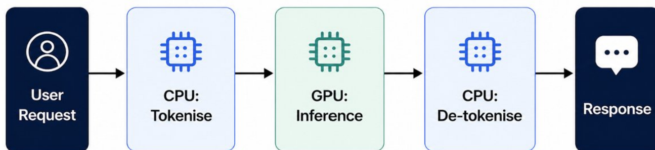
Figure 3: Chatbot inference workflow
