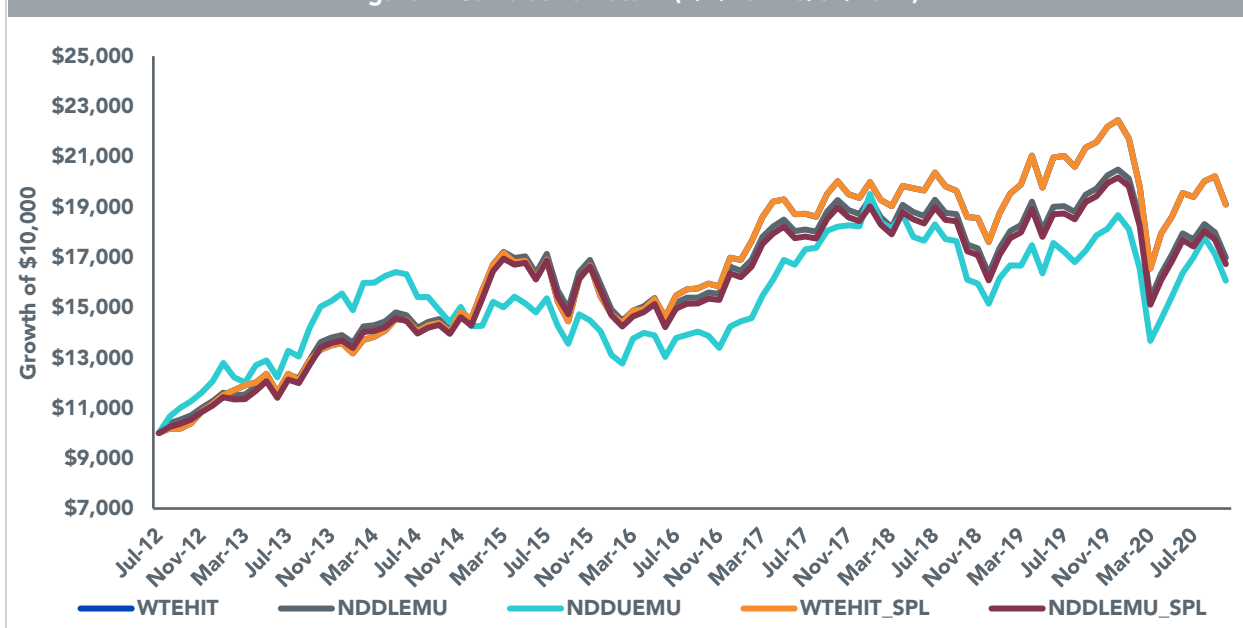
Figure 2: Cumulative Return (7/2/2012-3/31/2022)
